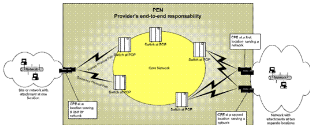
Figure 1 - Possible network lay-out for ANSPs connection to PENS.
