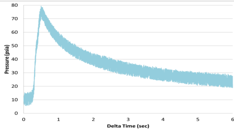
Test without suppression
