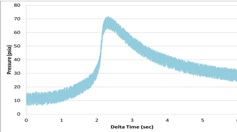
Test with 5.28% Halon
