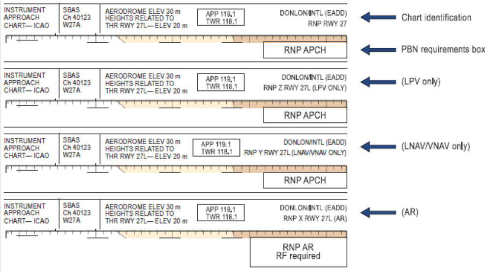
Figure 1-1. Example of new PBN chart designation (with PBN requirements box)
