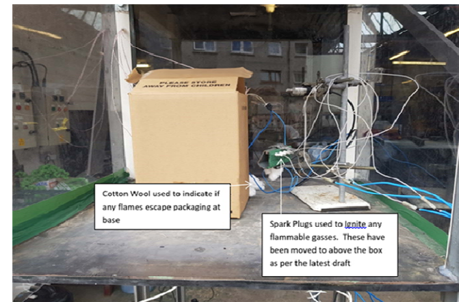
Setup of spark ignitors and cheesecloth
