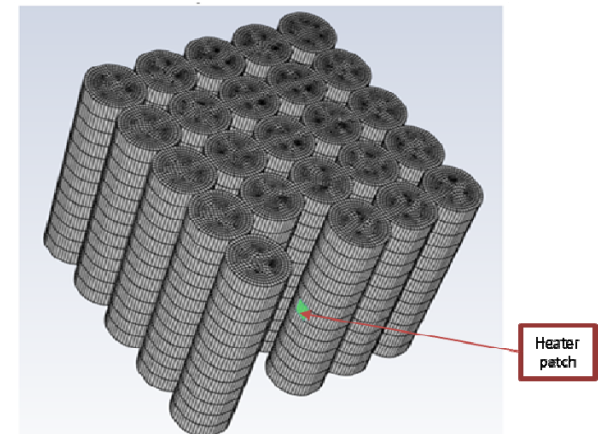
Computational domain for simulating IS experiments
